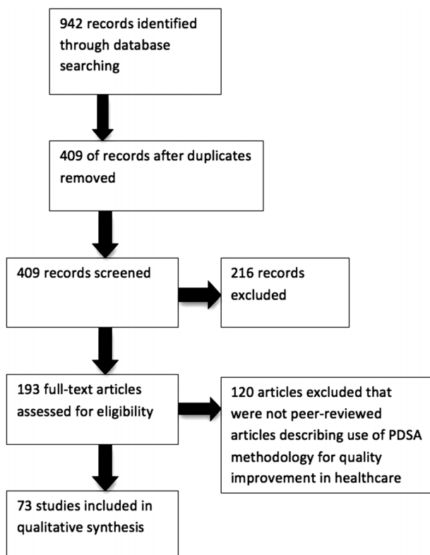
Figure 2 PRISMA diagram.
